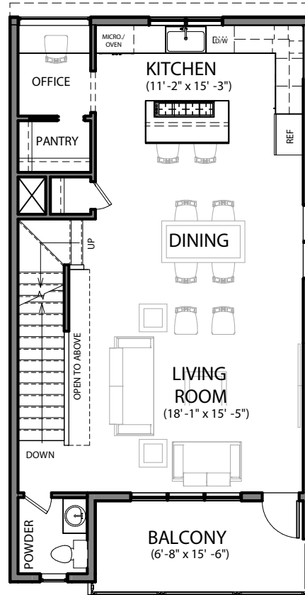
SECOND FLOOR 785 SF
