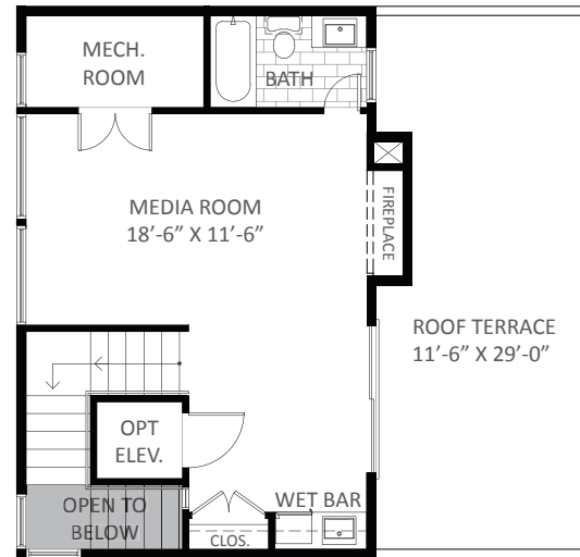
FOURTH FLOOR
