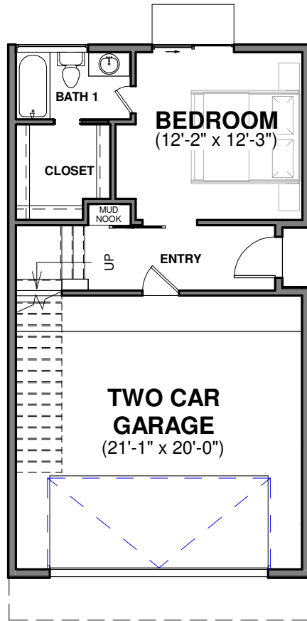
FIRST FLOOR 383 SF
