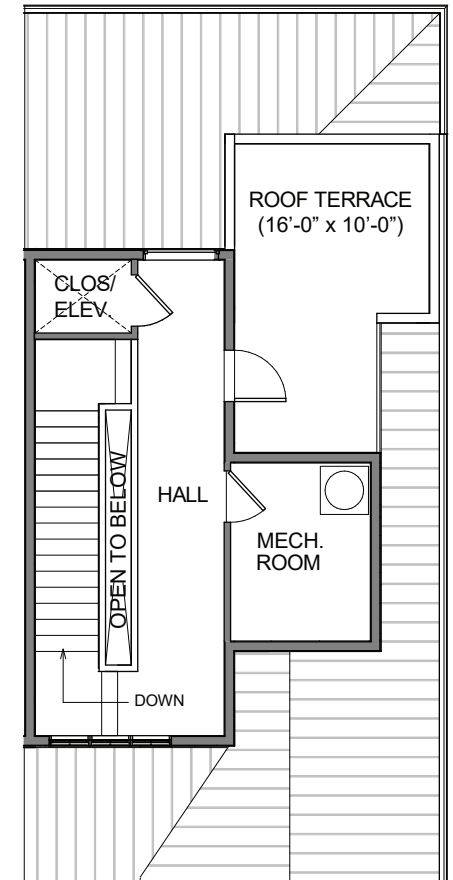
Roof Terrace
