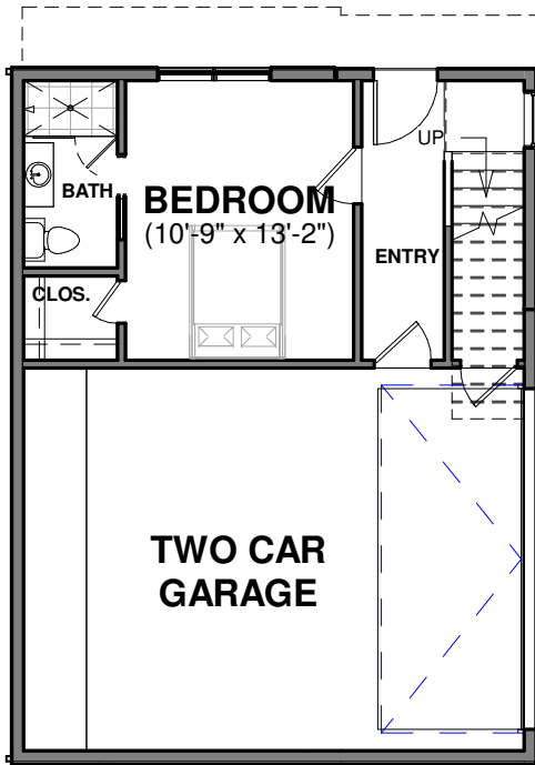
FIRST FLOOR 322 SF
