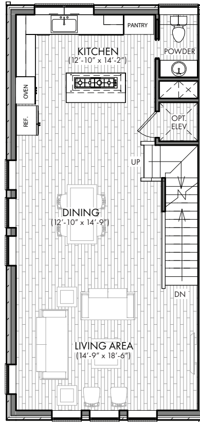
SECOND FLOOR 836 SF
