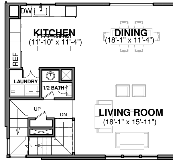
SECOND FLOOR 898 SF
